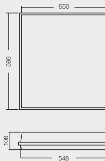
All dimension are in mm. Tolerance \pm 2 mm
