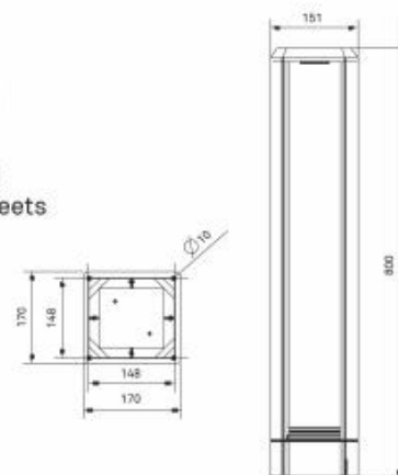
DIMENSION DRAWING
